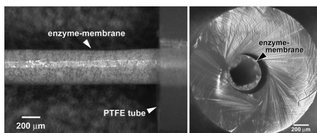
Figure 3. CCD images of a) cylindrical enzyme-membrane (dry state) exposed from the PTFE tube, which forms on the inner wall of the tube and b) a sectional view of the obtained CEM.
