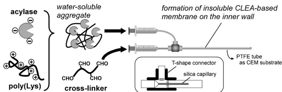
Figure 2. Schematic illustration of the procedure used to prepare an acylase-CEM. The cross-linking polymerization was performed in a concentric laminar flow. A silica capillary was fitted to the outer diameter of the T-shape connector by attaching to a PTFE tube using heat-shrink tubing. The capillary was set in the connector located at the concentric position of the CEM tube. The cross-linker solution was supplied to the substrate PTFE tube through the silica capillary, corresponding to a central stream in the concentric laminar flow. A solution of acylase-poly(Lys) mixture was poured from the other inlet of the T-shape connector, and formed an outer stream of the laminar flow.
