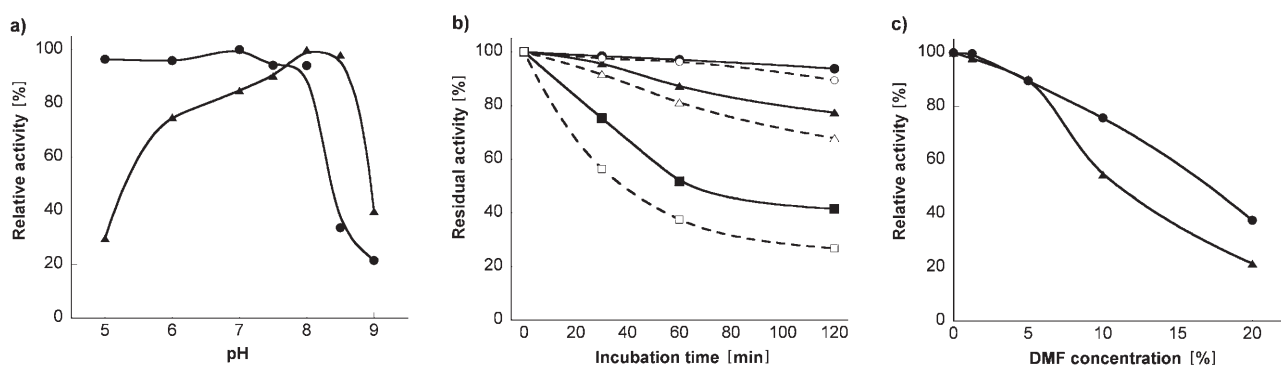
Figure 5. (a) Effect of pH on the enzymatic activity of the acylase-CEM (●) and the free acylase (▲). The activities at the pH optima were assigned values of 100%. (b) Temperature dependence of the enzymatic activity of the acylase-CEM (solid lines) and free acylase (dashed lines) at 40°C (circles), 50°C (triangles), and 60°C (squares). The activities without pre-incubation were assigned values of 100%. (c) Effect of organic solvent on the enzymatic activity of the acylase-CEM (●) and the free acylase (▲). The activities without organic solvent were assigned values of 100%. In all enzyme assays, 4 mM Ac-D,L-Phe was used as substrate.
