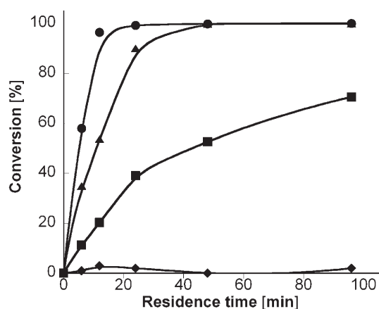
Figure 4. Hydrolysis of Ac-D,L-Phe in the acylase-CEM. A solution of substrate in Tris buffer (pH 8.0) was charged into a CEM tubing (inner volume = 24 \mu L) for various residence times. The reactions were carried out at three substrate concentrations [4 mM (●), 20 mM (▲), and 100 mM (■)] at 40°C. This acylase-based reaction converted the L-isomer only. A PTFE tube passed through a mixture of acylase and poly(Lys) had no enzymatic activity (◆).
