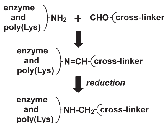
Scheme 1. Reaction of enzyme amino groups and/or poly(Lys) with aldehyde groups of the cross-linker.
