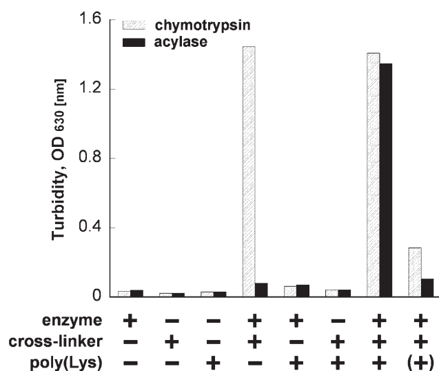
Figure 1. Effect of poly(Lys) on CLEA formation for electropositive chymotrypsin and electronegative acylase. Each bar shows the turbidity of the suspensions after incubation for 60 min at 4°C. A high turbidity means effective formation of the CLEA. The addition of each solution is described as “+” for each reagent and “-” for buffer without reagents. “(+)” indicates the addition of lysine instead of poly(Lys).
